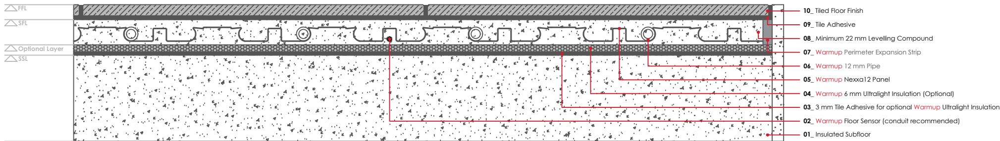
WARMUP NEXXA12 SYSTEM. Tiled floor finish
