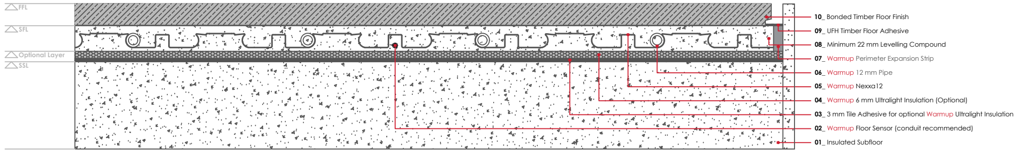
WARMUP Nexxa12 Bonded timber floor finish
