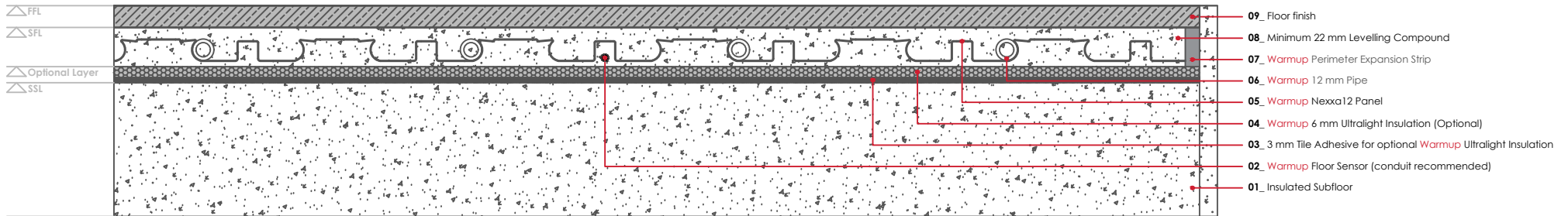
WARMUP NEXXA12 SYSTEM. Standard Detail
