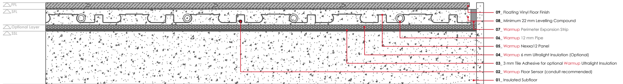
WARMUP Nexxa12 SYSTEM. Vinyl floor finish - floating
