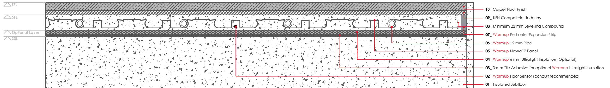
WARMUP Nexxa12 SYSTEM. Carpet floor finish
