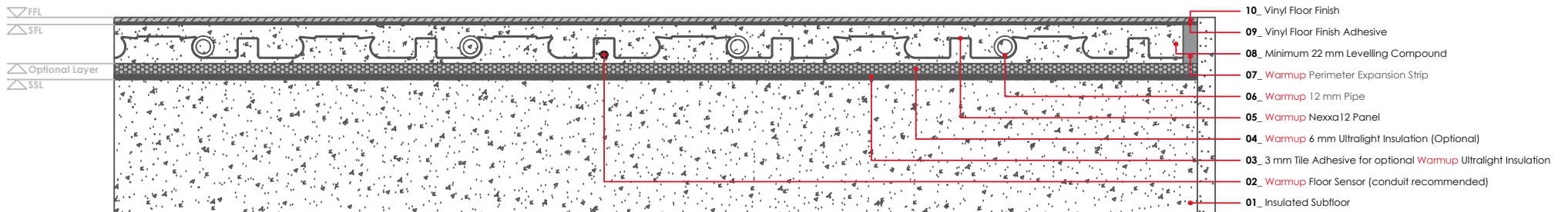
WARMUP Nexxa12 SYSTEM. Vinyl floor finish - glued
